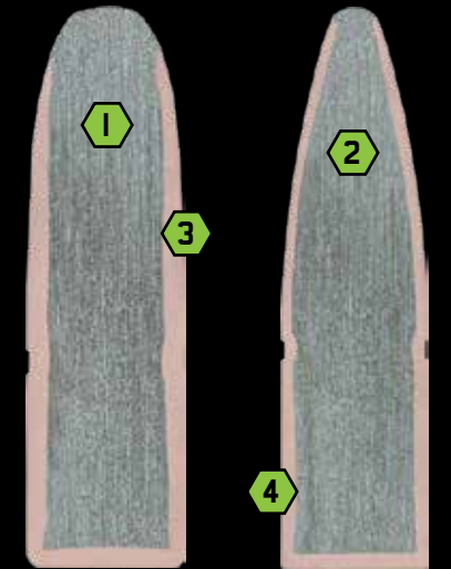
CORE-LOKT® SOFT POINT
